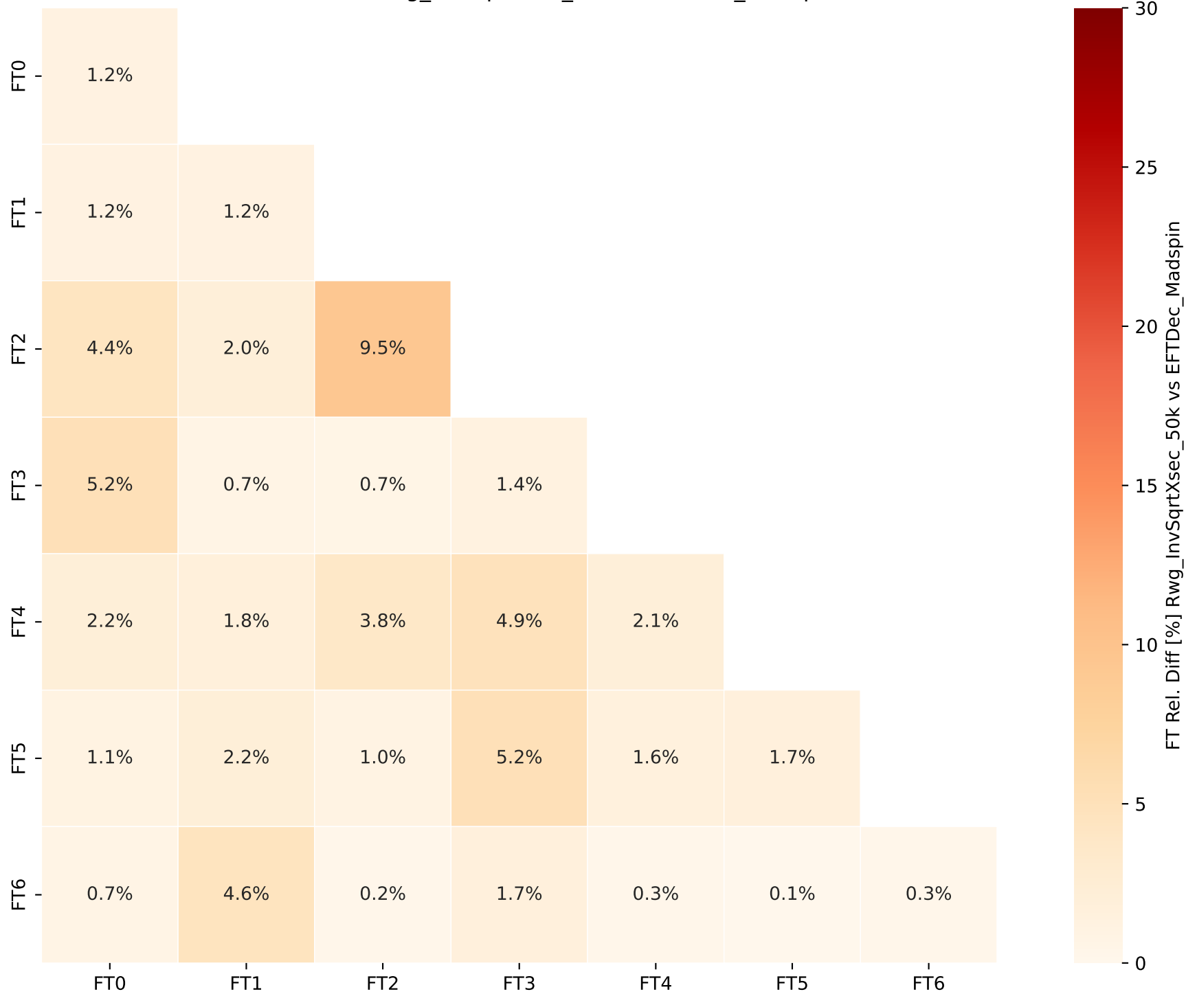
FT Rel. Diff [%] Rwg_InvSqrtXsec_50k vs EFTDec_Madspin
